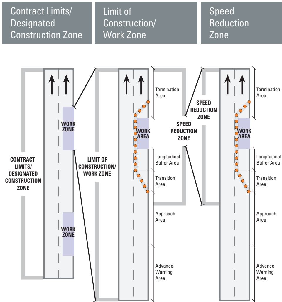
Figure 3.1 Component Areas
